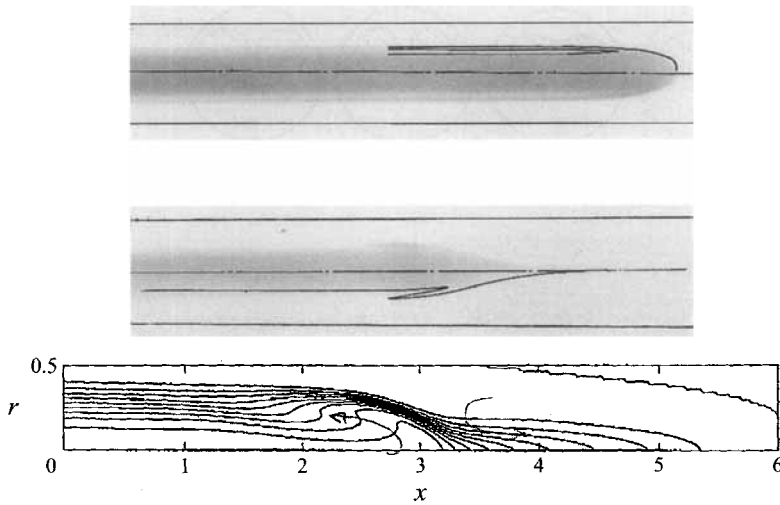
FIGURE 12. Partially enhanced photographs of the finger tip, indicating the reversed flow that exists at the nose, under some circumstances when m < 0.5 . The line drawing is from Part 2 for a situation similar to that shown in the lower photograph.
