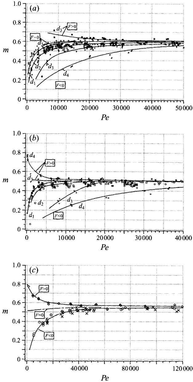
FIGURE 6. (a) The diagnostic quantity, m , versus Péclet number ( Pe ), for At = 0.985 and tubes of the various stated diameters set vertically, i.e. d_1 indicates a diameter of 1 mm etc. Here F > 0 for the case of glycerine above the mixture and F < 0 for the inverse. Here, as in all the graphs that follow, the lines were inserted by eye, based on considerable experience. Readers are invited to supply their own versions as needed. (b, c) The same as (a) but for At = 0.43 and 0.79 respectively. In (c) all curves are for a tube diameter of 3 mm and the interpolated curve for F = 0 is shown also (cf. figures 9(a) and 9(b) for At = 0.785 and 0.43 respectively).
