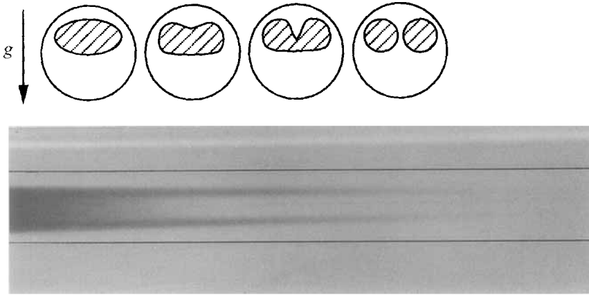
FIGURE 10. Finger splitting in a horizontal, 4 mm tube with the displacing fluid lighter than that displaced. The sketches indicate the cross-section of the instability at various locations along its length.
